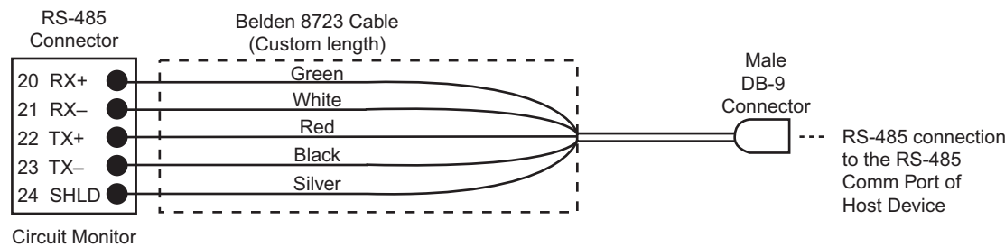
Figure 6–6: Typical procedure for connecting the first device on the daisy chain
