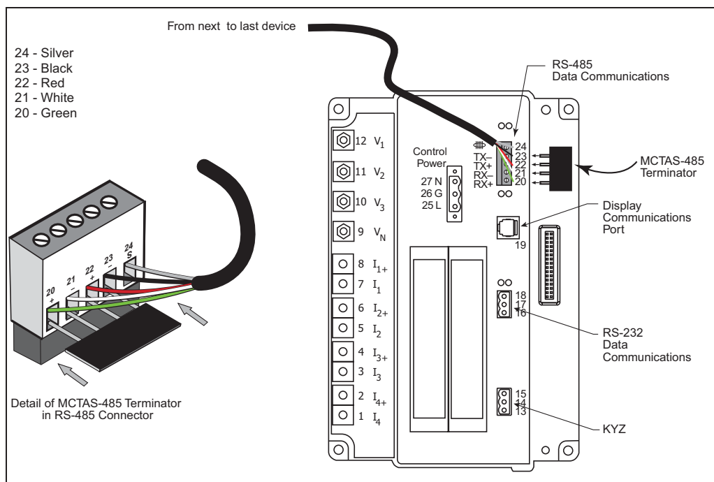
Figure 6–7: Terminating the circuit monitor using the MCTAS-485 terminator
